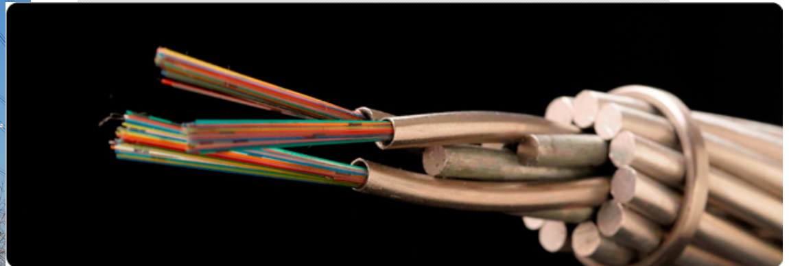
Multi Loose Tube Type
